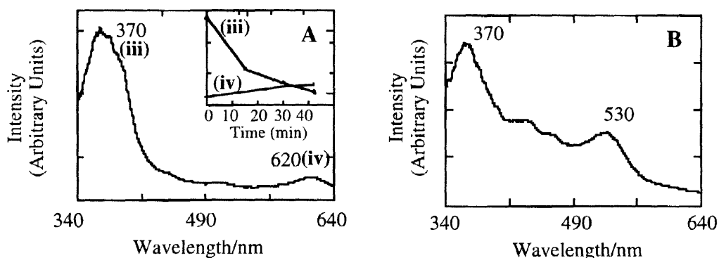
Figure 3. A) DR (1/R) of 1b adsorbed onto HZSM-5 zeolite at reflux of isooctane (The inset shows the decay and growth profiles of bands (iii) and (iv)). B) DR (1/R) of 1b adsorbed onto HY zeolite at reflux of isooctane.
