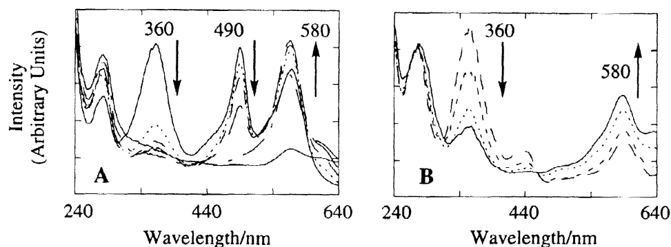
Figure 1. DR spectra (taken every hour) of 1a adsorbed onto A) HY zeolite and B) HZSM-5, showing the kinetic of disappearance and growing of the different intermediate species. For assignment see Scheme 1.
