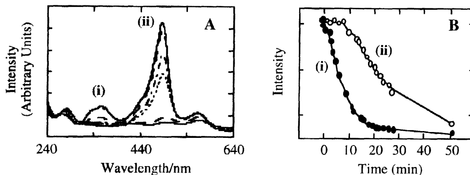
Figure 2. A) DR (1/R) of 1a adsorbed onto HY zeolite at reflux of hexane. B) Normalized decay profiles of bands (i) and (ii) of Figure 2A.
